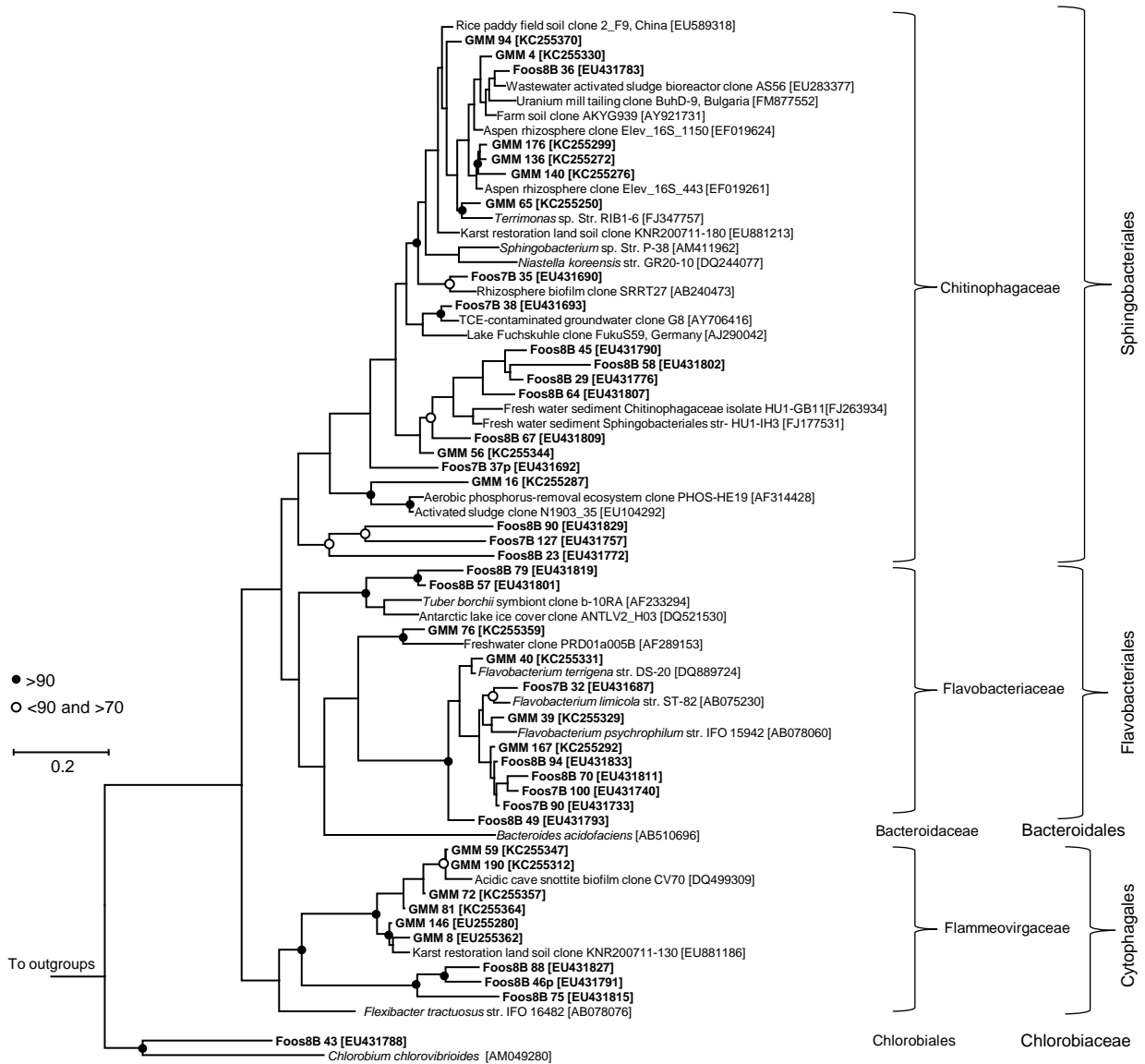
Supplemental Figure 4. Phylogenetic reconstruction among 16S rRNA gene sequence retrieved from moonmilk from Grotta della Foos and Bus della Genziana (labeled in bold) compared to closest relatives affiliated to the Bacteroidetes. Accession numbers for relatives are included. The scale bar corresponds to distance.
