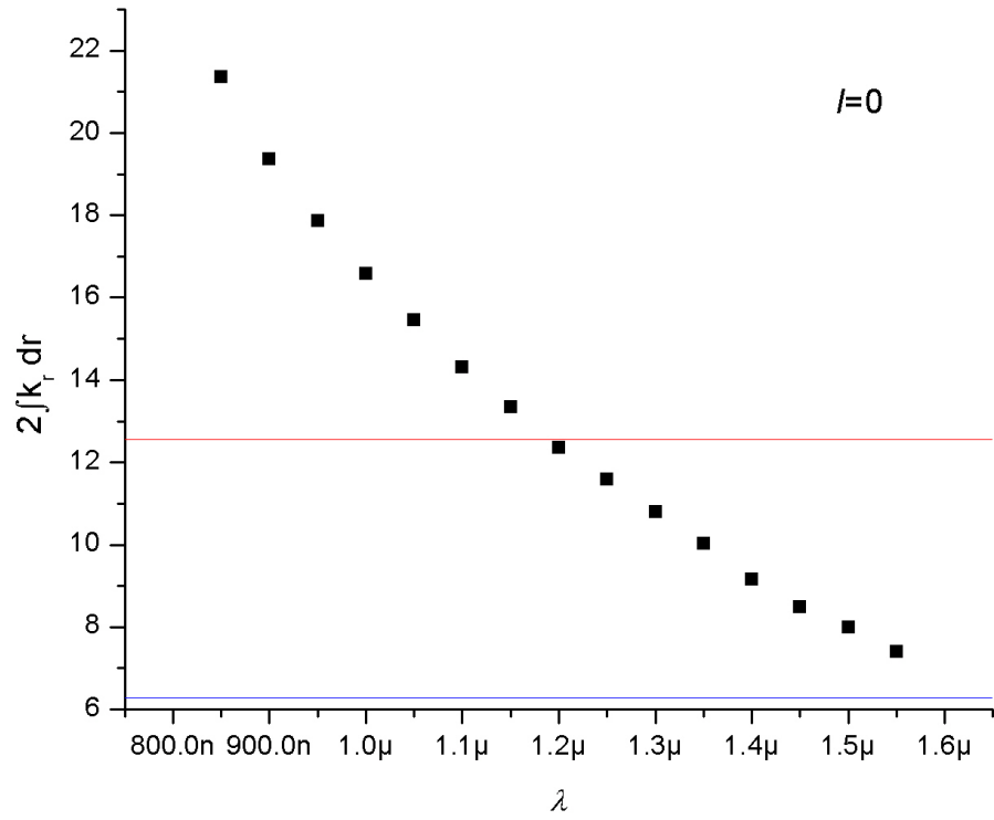
Figure 11: 2\int k_r dr vs. \lambda - for l = 0 ; Region of Only One Mode
