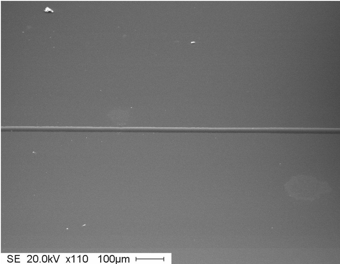
Figure 4: 1.7cm Segment of waveguide as seen with a Scanning electron microscope
