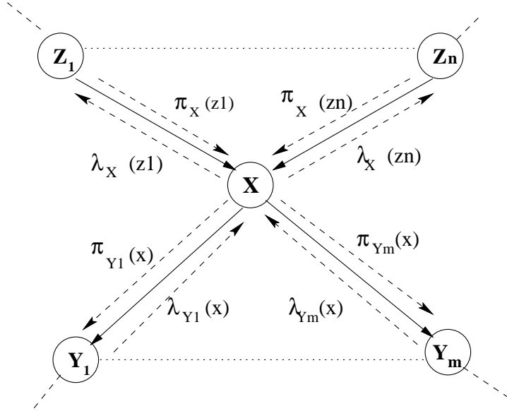
Figure 4.1. Probabilistic Inference Using Local Message Passing.
