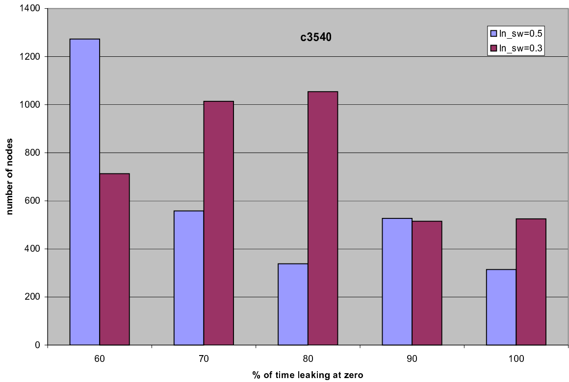
Figure 5.5. Graph Showing the Break-up of Leakage Profile for Different Switching Profile for c3540.
