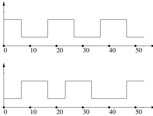
Figure 1.5. Two Different Signals having Identical Frequency [3].
