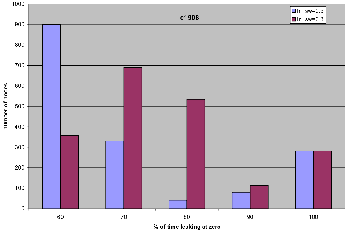
Figure 5.4. Graph Showing the Break-up of Leakage Profile for Different Switching Profile for 1908.
