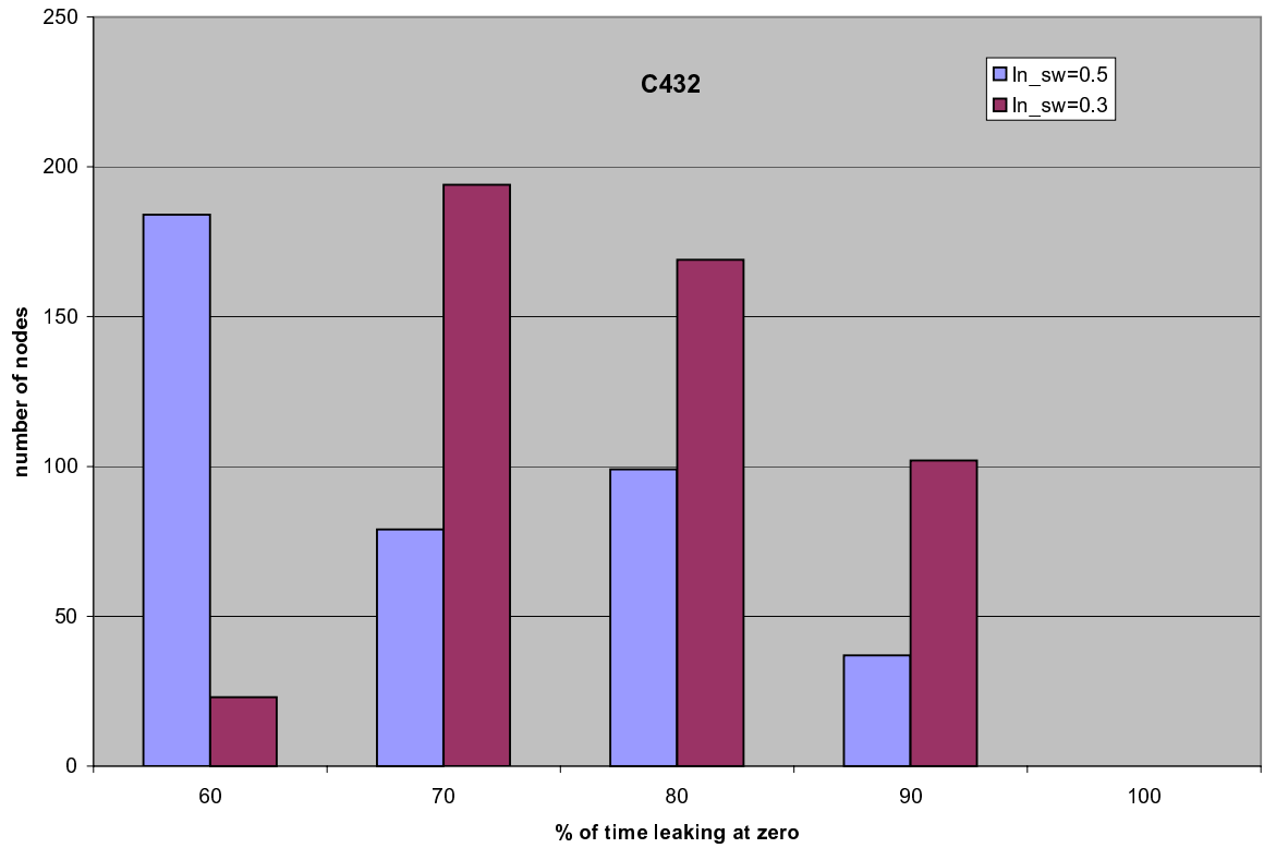
Figure 5.3. Graph Showing the Break-up of Leakage Profile for Different Switching Profile for c432.
