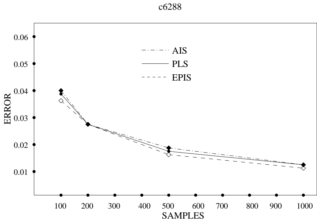
Figure 4.4. Graph Showing the Time Accuracy Trade-off for c6288.
