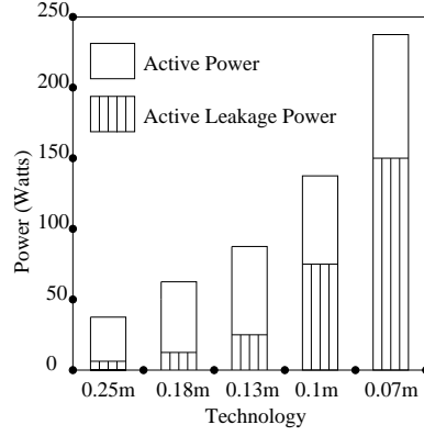
Figure 5.1. Graph Showing Rise in Leakage Power with Technology [1].
