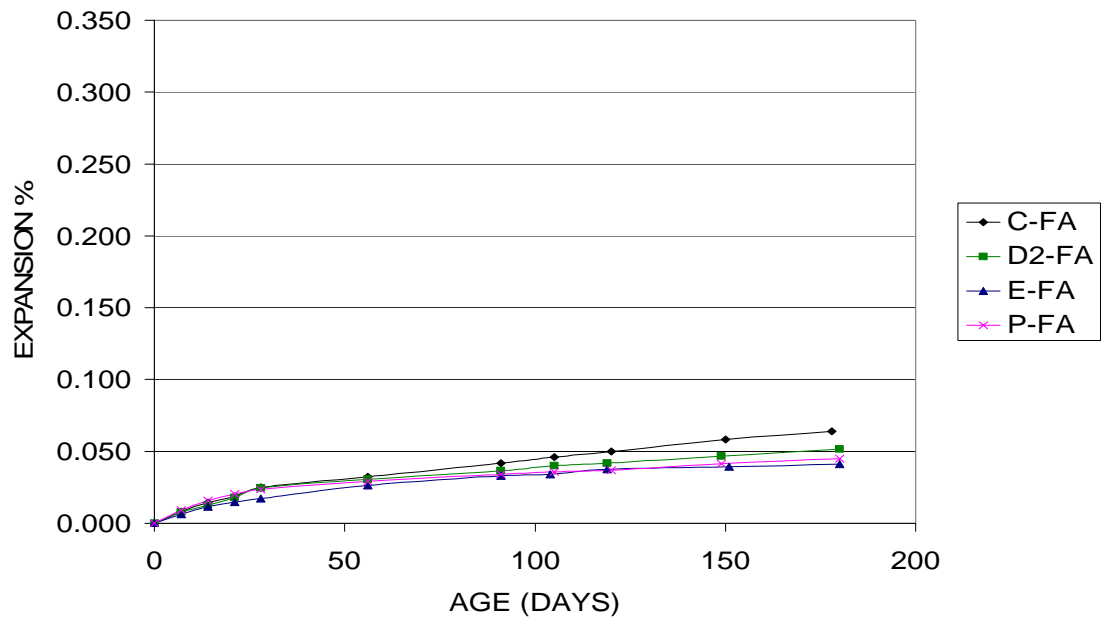
Figure 32. Expansion versus Age for the Cements with 20% Replacement by Fly Ash
