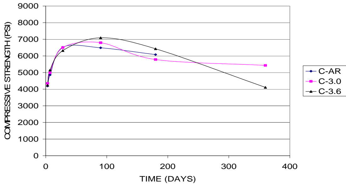
Figure 4. Compressive Strength versus Age for C, C-3.0, and C-3.6 in Sulfate
