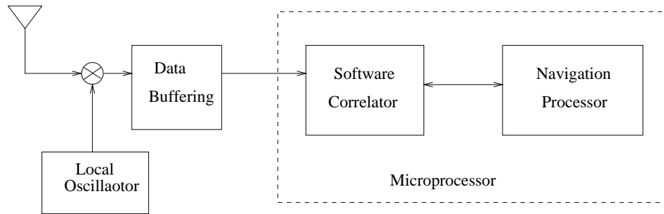
Figure 1.1. Software GPS Receiver
