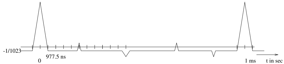
Figure 2.15. C/A Code Autocorrelation
