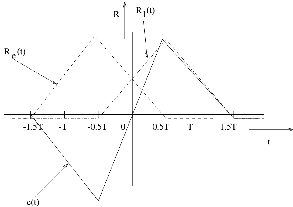
Figure 2.8. S-Curve
