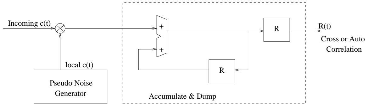
Figure 4.6. Digital Implementation of Serial Correlator
