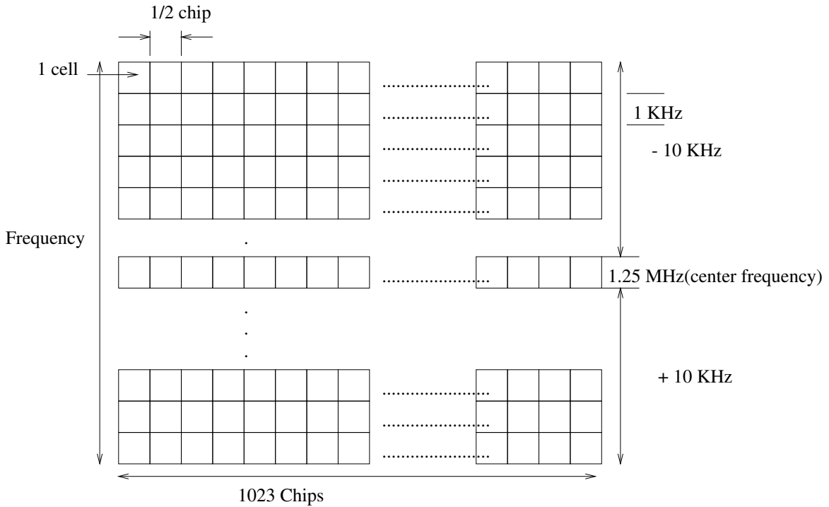
Figure 2.4. Two Dimensional Acquisition Search Space
