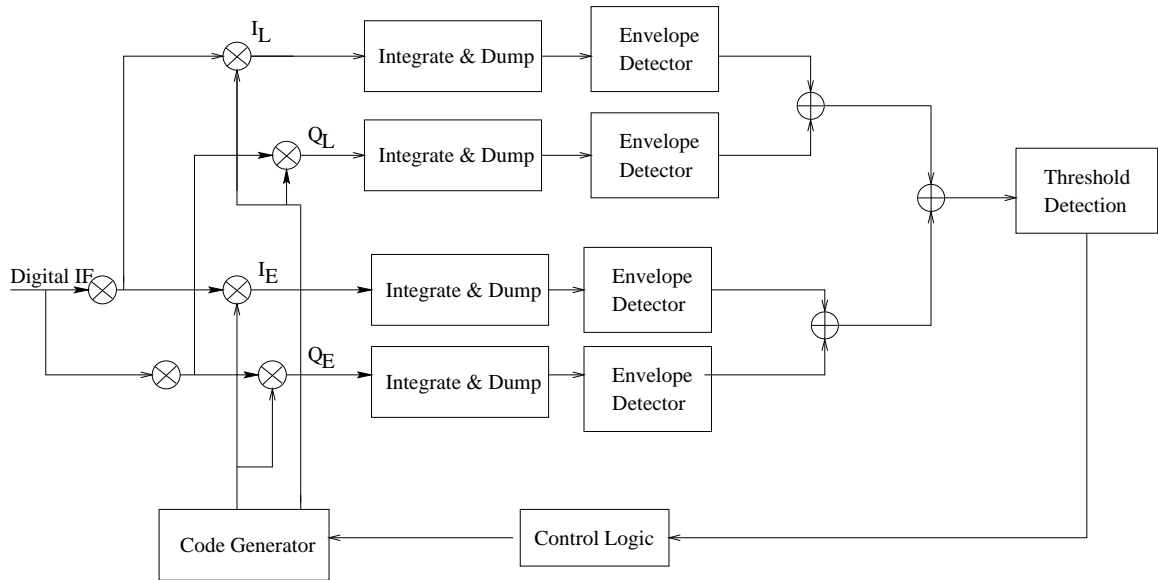
Figure 3.5. Tracking Loops
