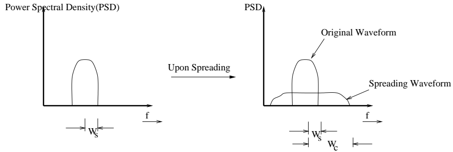
Baseband BW W_s spread by a sequence of BW W_c . The Power Spectral Density (PSD) is plotted versus frequency.
