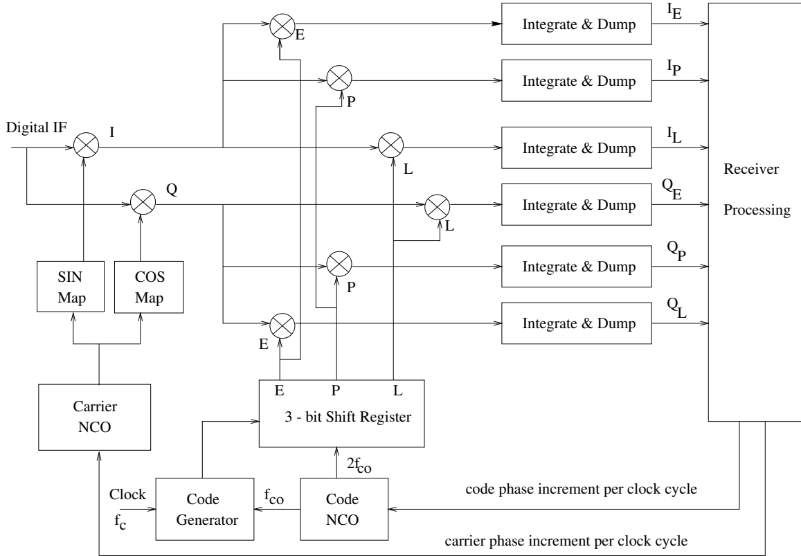
Figure 3.2. Digital Receiver Channel
