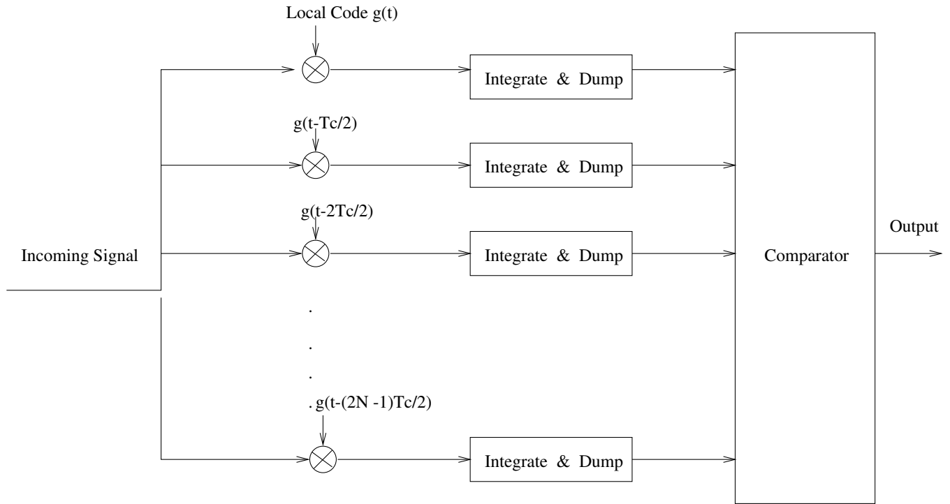
Figure 2.6. Parallel Correlator
