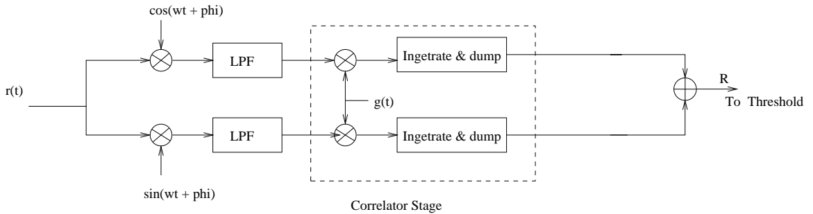
Figure 2.10. Coherent Demodulation
