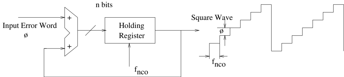
Figure 4.3. Numerical Controlled Oscillator
