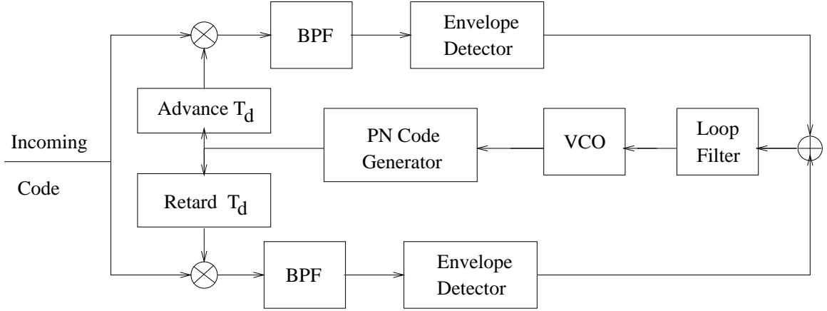
Figure 2.7. Delay Locked Loop
