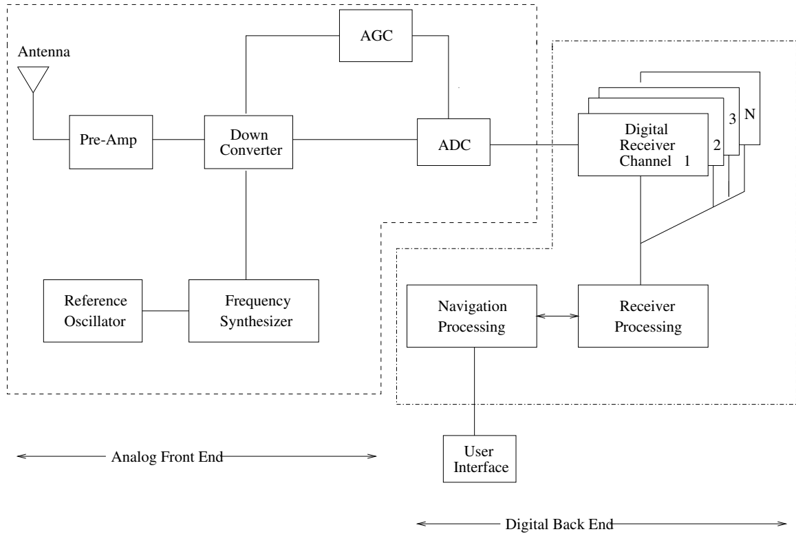
Figure 3.1. GPS Receiver
