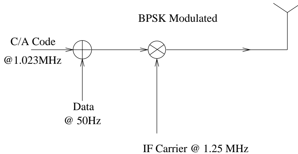
Figure 4.5. IF GPS Signal Generation
