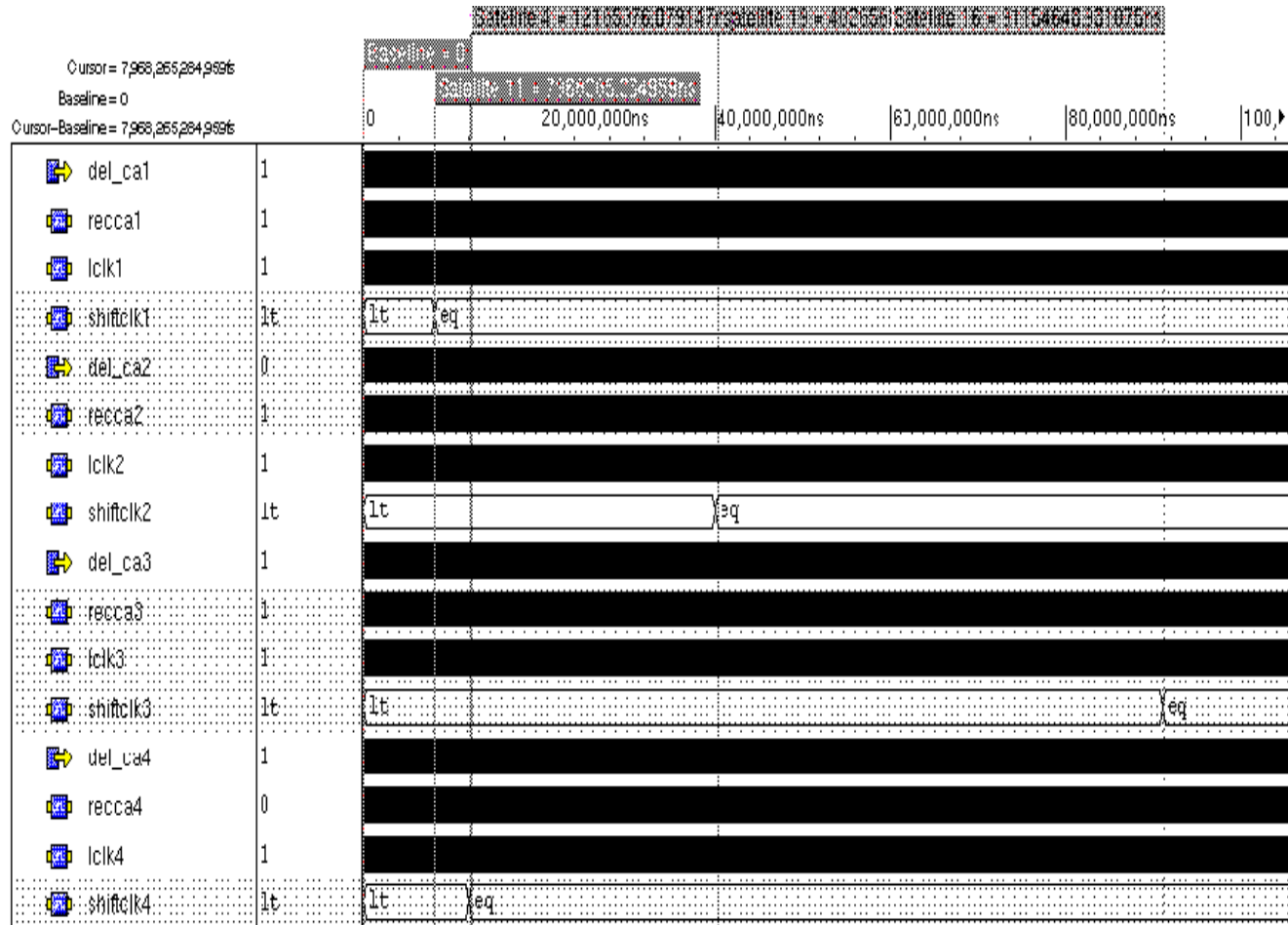
Figure 5.14. Acquiring Multiple Satellites Set 2
