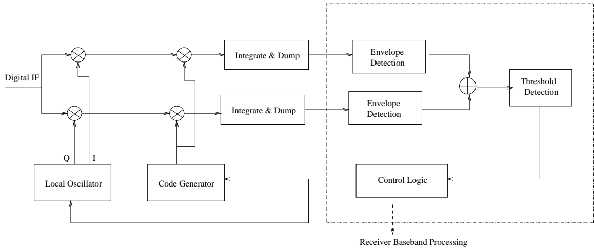
Figure 3.3. Channel Serial Acquisition
