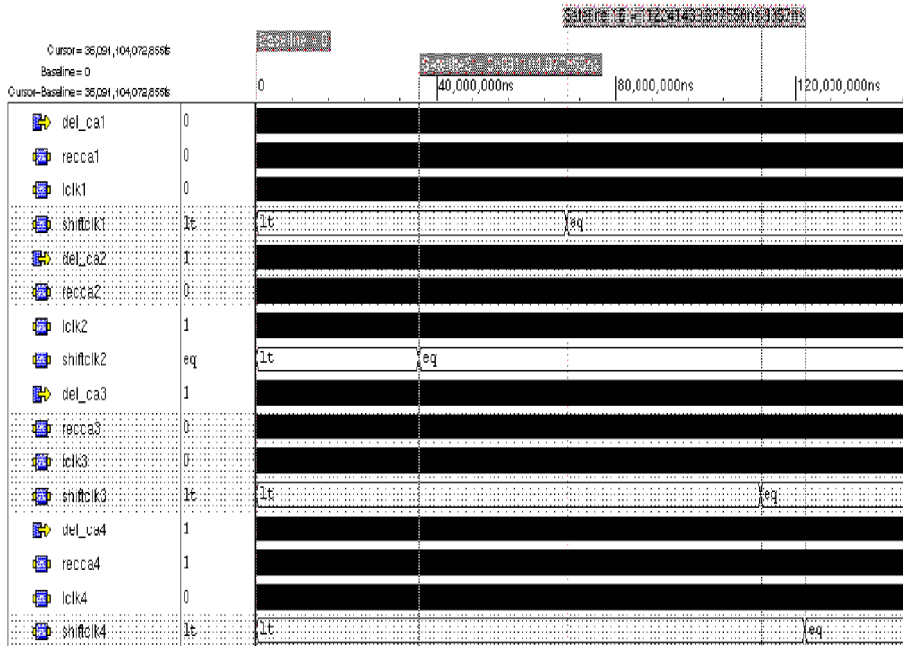
Figure 5.15. Acquiring Multiple Satellites Set 3
