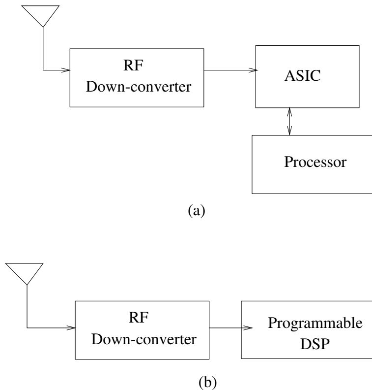
Figure 1.2. Receiver Block Diagrams: (a) Hardware (b) Software
