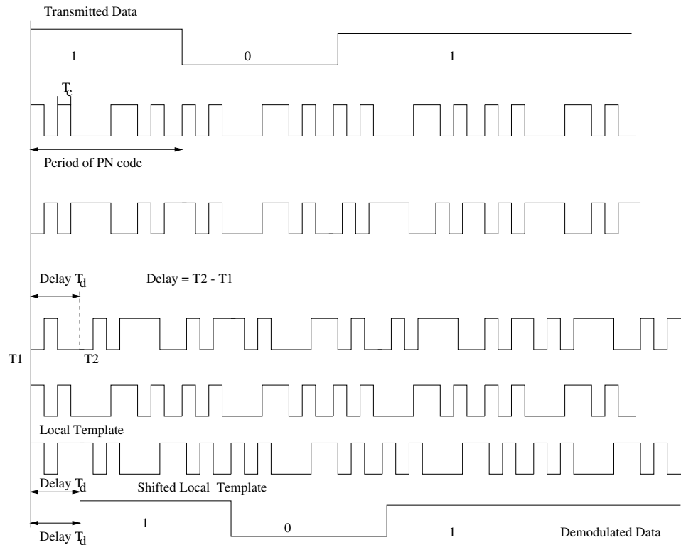
Figure 2.16. Position Determination using Pseudo-codes
