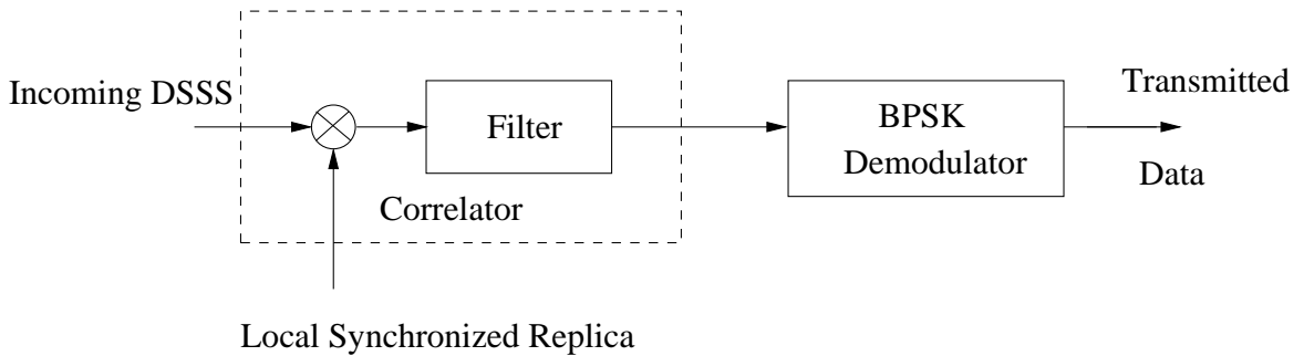
Figure 2.3. Direct Sequence Demodulator
