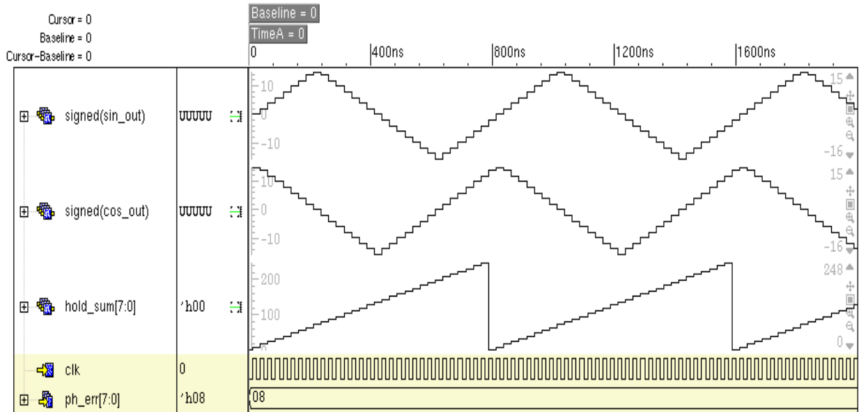
Figure 5.1. Sine Wave Generation
