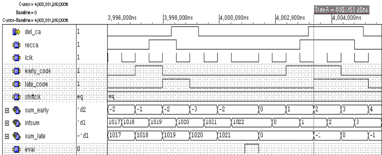
Figure 5.12. Tracking After Signal has been Acquired
