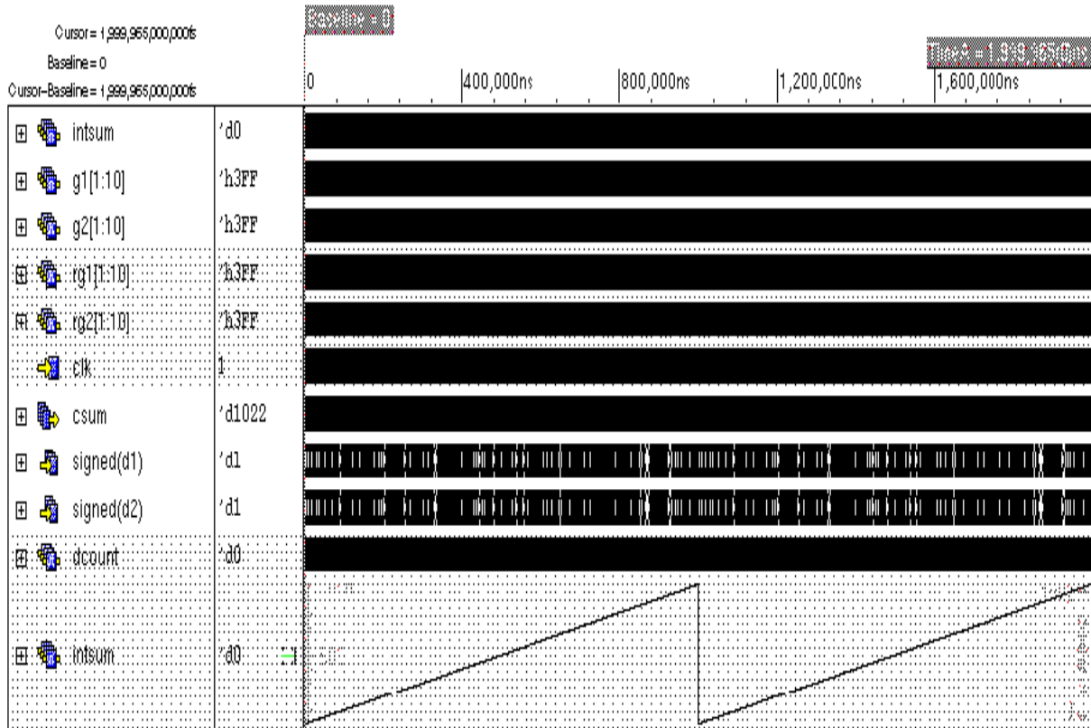
Figure 5.3. Auto Correlation using Accumulate and Dump
