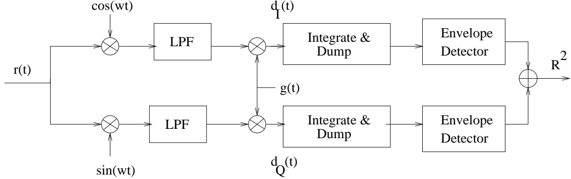
Figure 2.9. Non-coherent Demodulation
