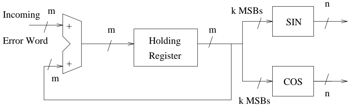
Figure 4.4. Direct Digital Frequency Synthesizer
