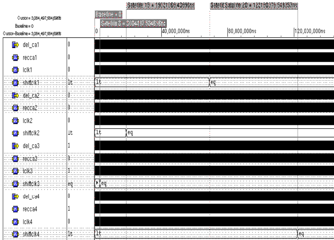
Figure 5.16. Acquiring Multiple Satellites Set 4
