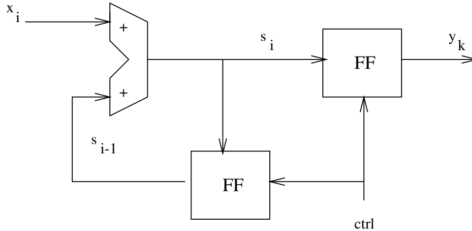
Figure 4.1. Integrate and Dump
