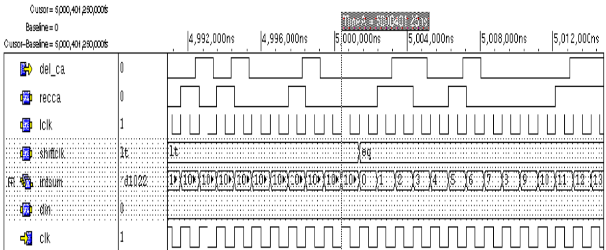
Figure 5.11. Acquisition of a Single Satellite by Incrementing Code Phase in Half Chip Increments
