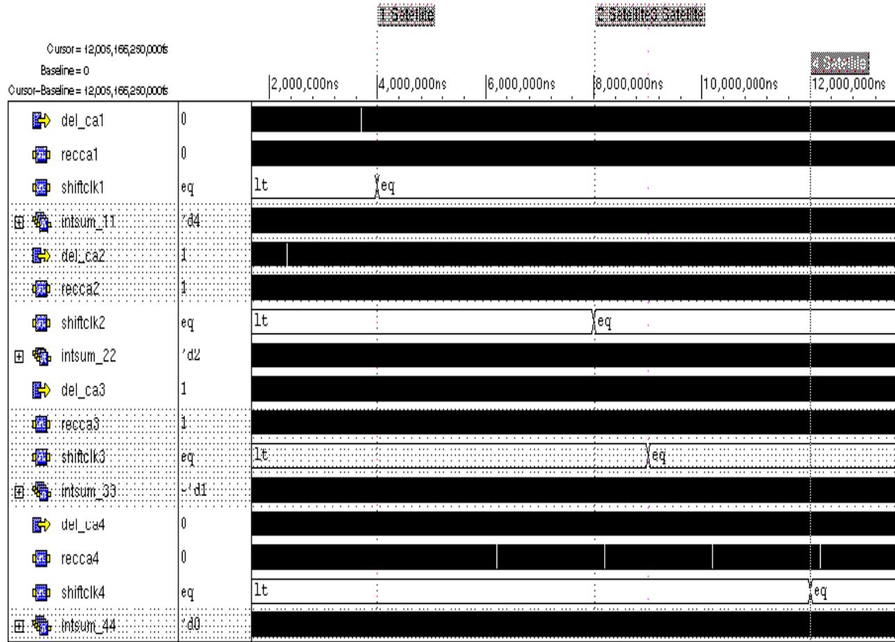
Figure 5.13. Acquiring Multiple Satellites Set 1
