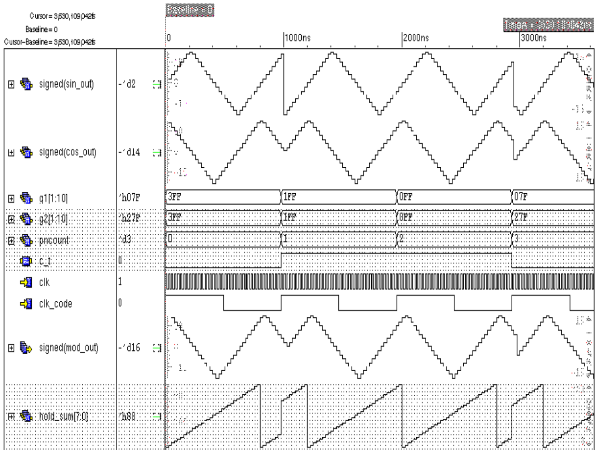
Figure 5.2. Binary Phase Shift Keying Signal
