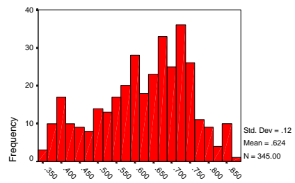
Histogram
