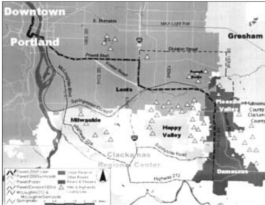
Figure 6. Alignment alternatives
