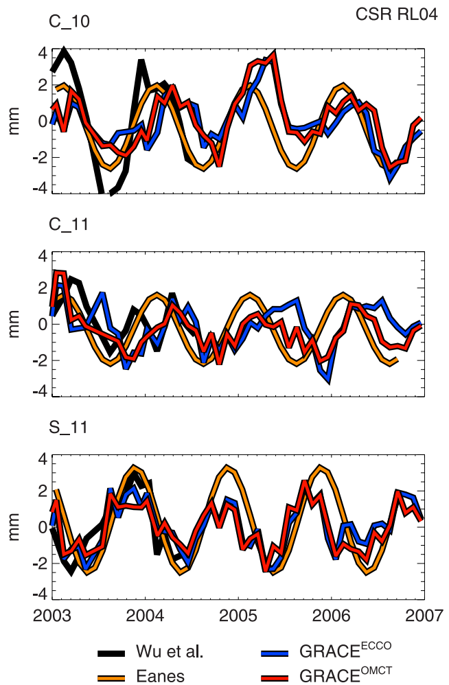
Figure 5. Same as Figure 3 except that here the monthly geocenter time series is GSM-like, in that it has had atmospheric and oceanic contributions removed corresponding to GRACE Level-2 data processing standard.
