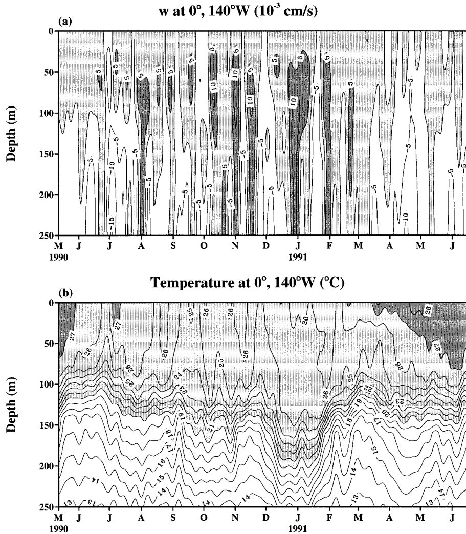
Figure 2. (a) Estimated vertical velocity component from the TIWE array and (b) temperature from the TAO array as functions of time and depth at 0°, 140°W. For vertical velocity, shading denotes upwelling, with dark shading denoting values in excess of 5 \times 10^{-3} cm s -1 , and the contour interval is 5 \times 10^{-3} cm s -1 . For temperature, shading denotes values larger than 20°C, with dark shading denoting values in excess of 27°C, and the contour interval is 1°C. All data were low-pass filtered to remove oscillations on timescales shorter than 10 days.
