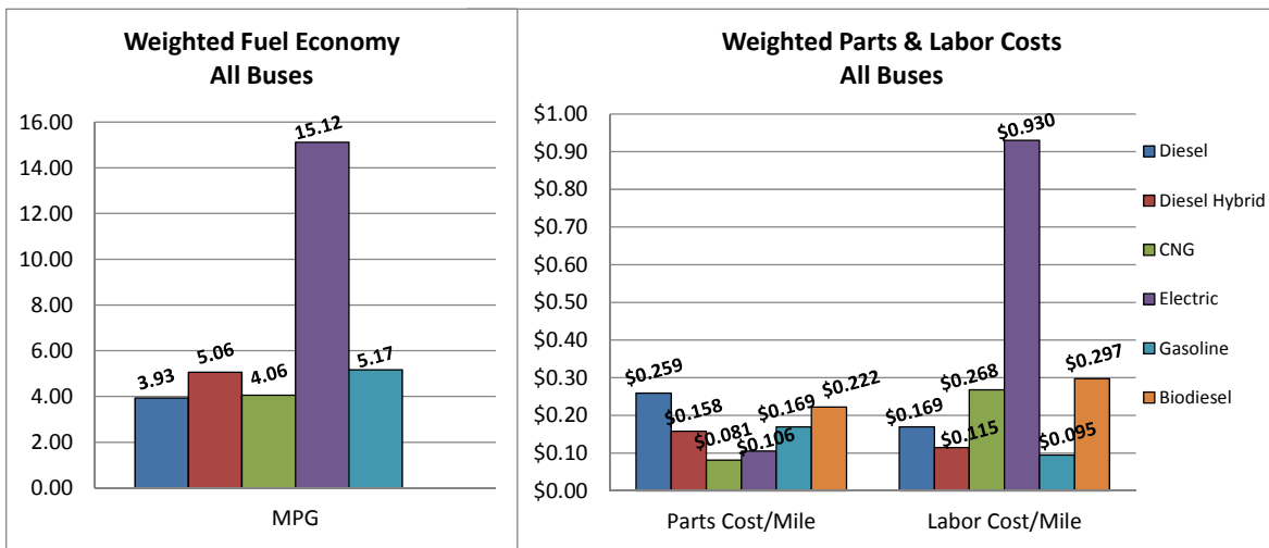
Figure 3-13. Weighted comparison – all propulsion types and bus sizes.
