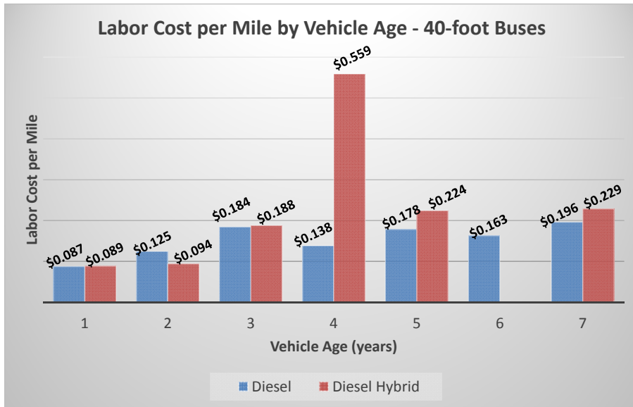
Figure 3-5. Comparison of labor cost per mile by vehicle propulsion and age – 40-foot buses.
