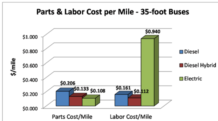
Figure 3-8. Operating cost comparison of different power plants – 35-foot buses.
