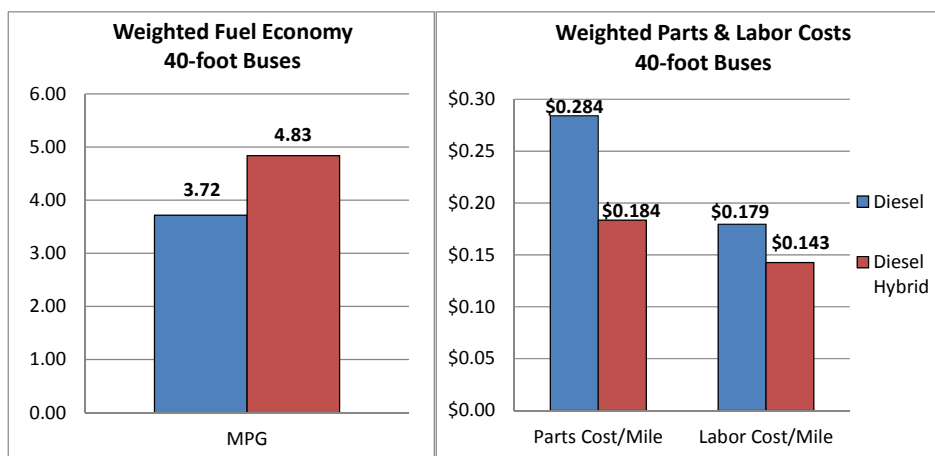
Figure 3-12. Weighted cost and performance comparison for 40-foot buses.
