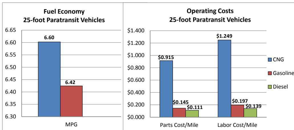
Figure 3-18. Comparison of performance and costs – 25-foot paratransit vehicles.
