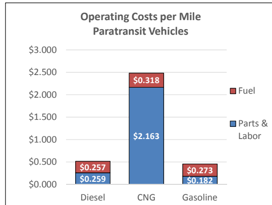
Figure 3-16. Comparison of operating costs per mile – paratransit vehicles.
