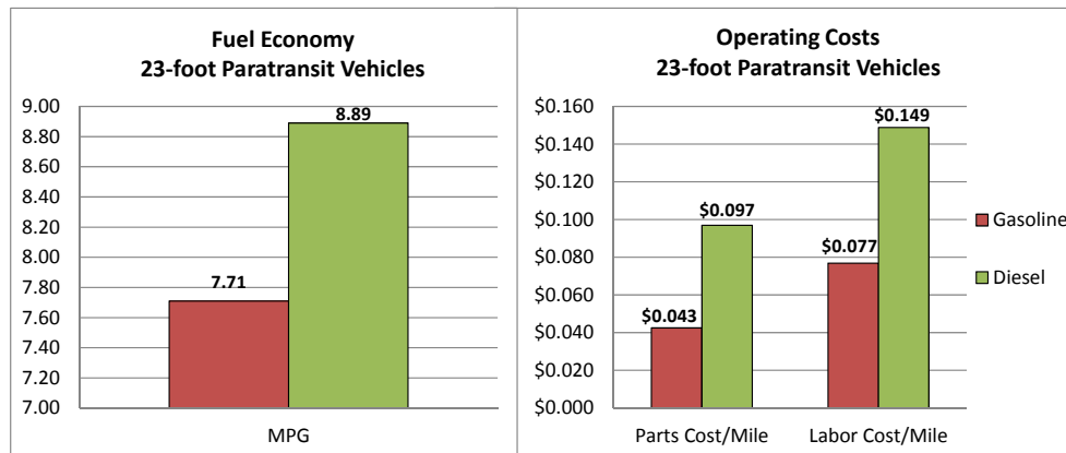
Figure 3-17. Comparison of operating costs – 23-foot paratransit vehicles.
