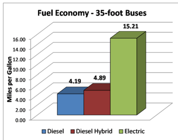
Figure 3-7. Fuel economy comparison of different power plants – 35-foot buses.
