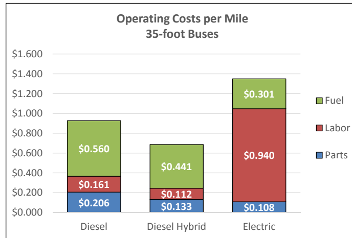
Figure 3-9. Comparison of operating costs for different power plants – 35-foot buses.
