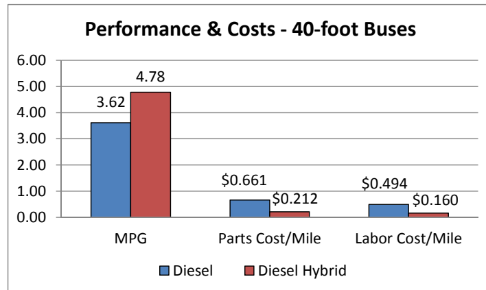
Figure 3-2. Comparison of performance and costs of 40-foot buses, diesel vs. diesel hybrid.
