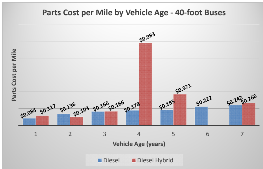
Figure 3-4. Comparison of parts cost per mile by vehicle propulsion and age – 40-foot buses.
