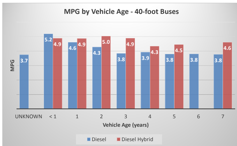
Figure 3-3. Comparison of fuel mileage by vehicle age – 40-foot buses.
