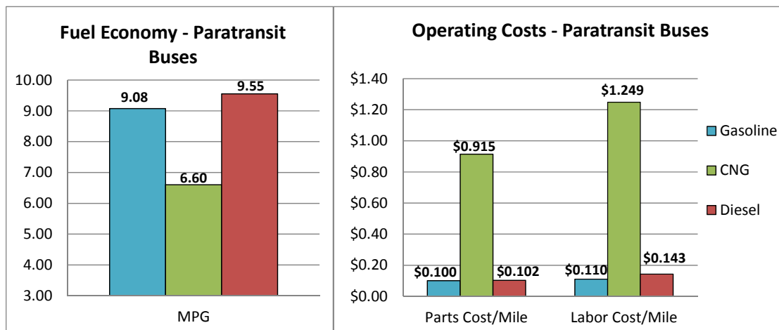
Figure 3-15. Comparison of paratransit vehicles with different power plants.
