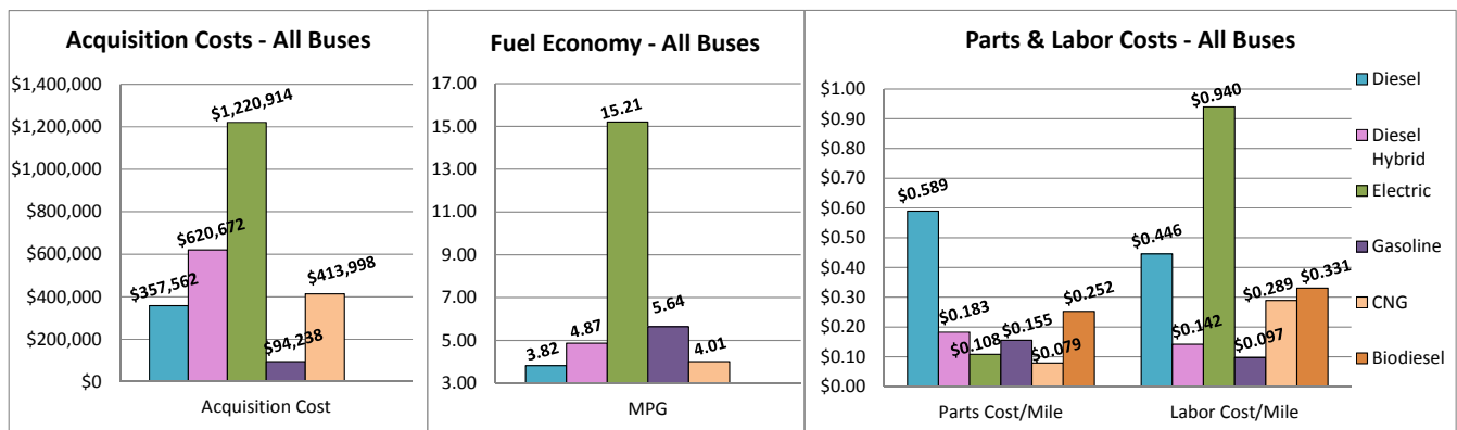
Figure 3-10. Comparison of buses with different power plants – all vehicle sizes.
