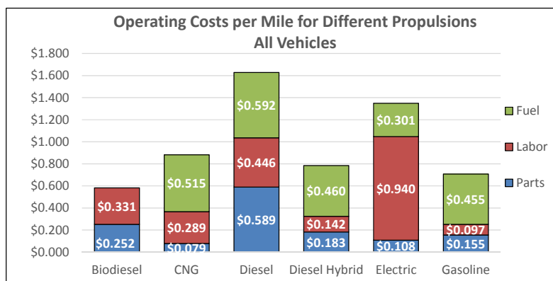
Figure 3-11. Comparison of operating costs between different power plants.
