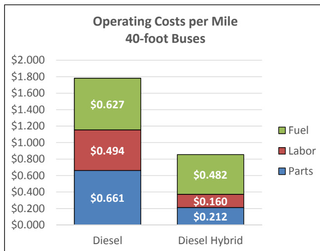
Figure 3-6. Comparison of operating costs for different power plants – 40-foot buses.
