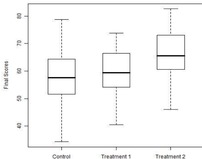
Figure 1: Boxplots of final scores adjusted for covariates for all treatment levels (Residuals were plotted after adding back adjusted means to each score). Control was administered during the spring and summer session. Treatment 1 was administered during the spring semester; Treatment 2 was administered during the summer semester.
