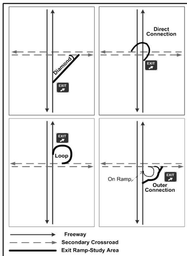
Figure 1. Four typical exit ramp types.
